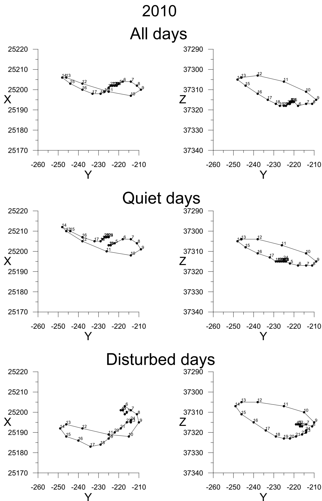
Fig. 4 Hodographs of the diurnal variation in the horizontal and vertical planes for all days, quiet days and disturbed days. Units are nT. Each point has its time label.
